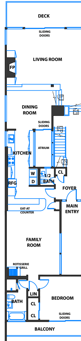
MAIN LEVEL
